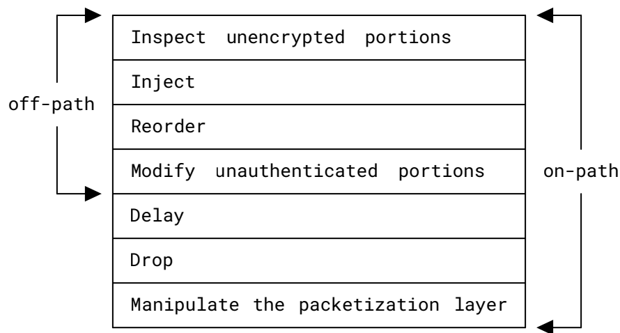
Figure 4: Attacker Capabilities
