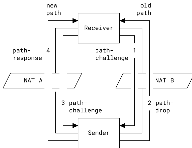
Figure 7: Old Path Is Not Preferred
